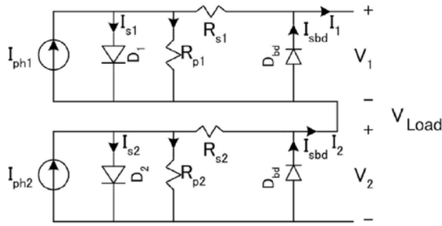
FIGURE 1. Electric circuit model of a PV module with two bypass diodes
